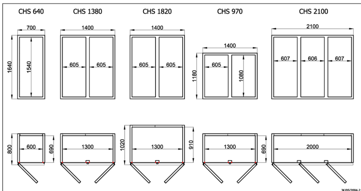
Drw. 1 – dimensioned sketch
